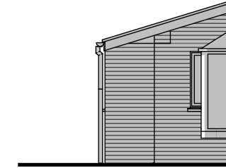
proposed single storey show entrance extension
